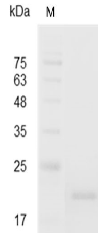
SDS-PAGE analysis of recombinant mouse IL-28A
